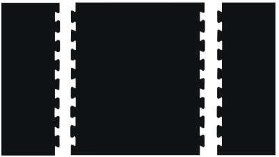
End piece Center piece End piece H 13 mm W 80 cm D 70/30 cm
