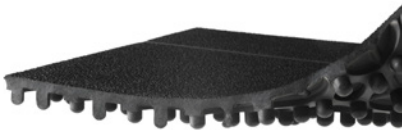
Bottom side. H 15 mm W 91 cm D 91 cm
